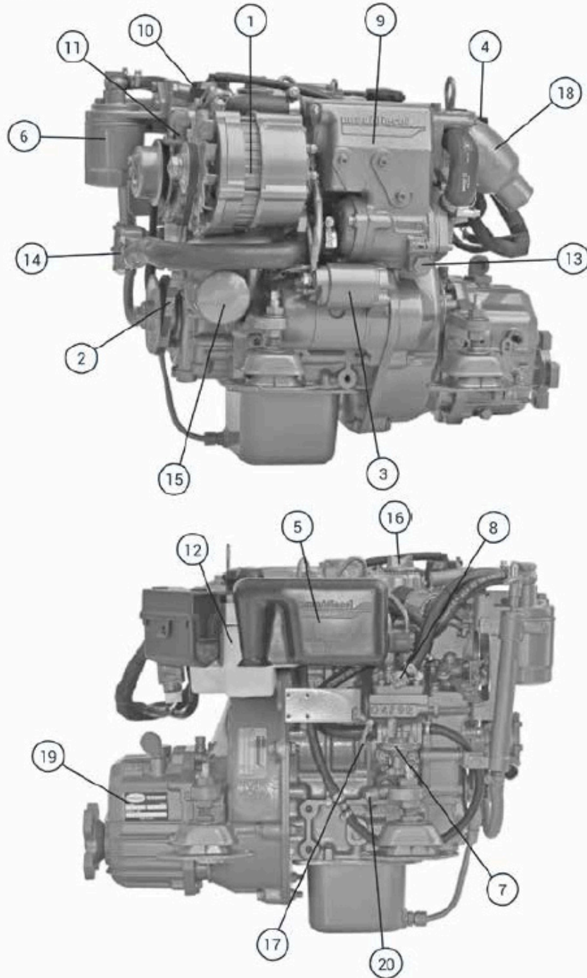
ENGINE VIEWS N3.21
