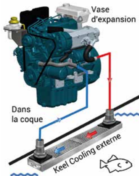
External keel cooling principle
