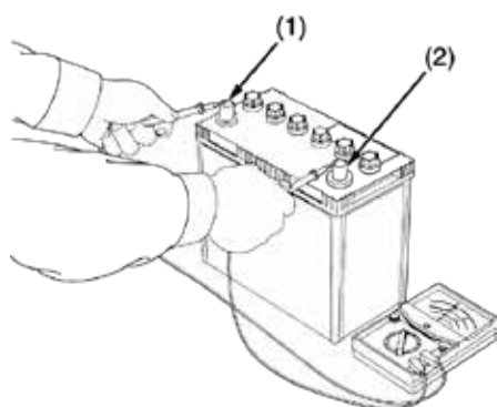
(1) Borne positive (2) Borne négative
